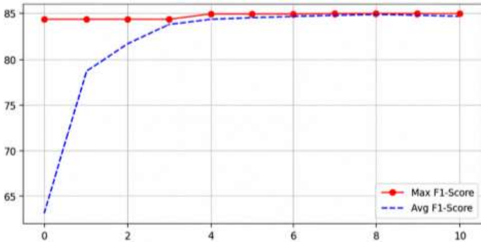
Figure 2. Convergence Plot of Maximum and Average Fitness Across 10 Generations
