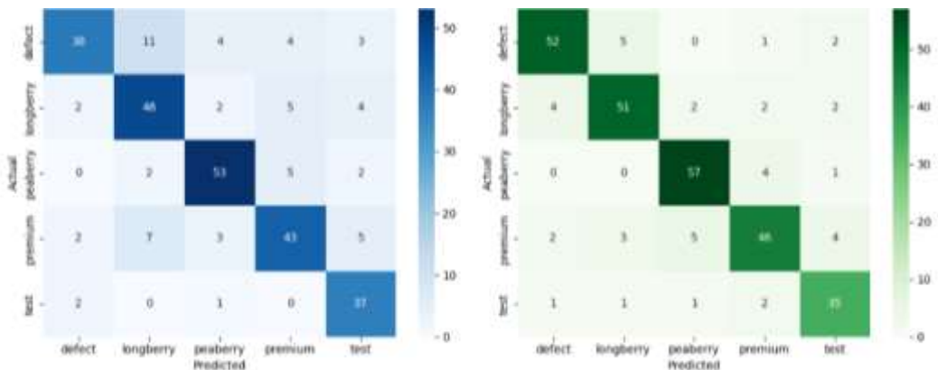
Figure 3. Confusion Matrix Comparison Between Default SVM and GA-Optimized SVM
